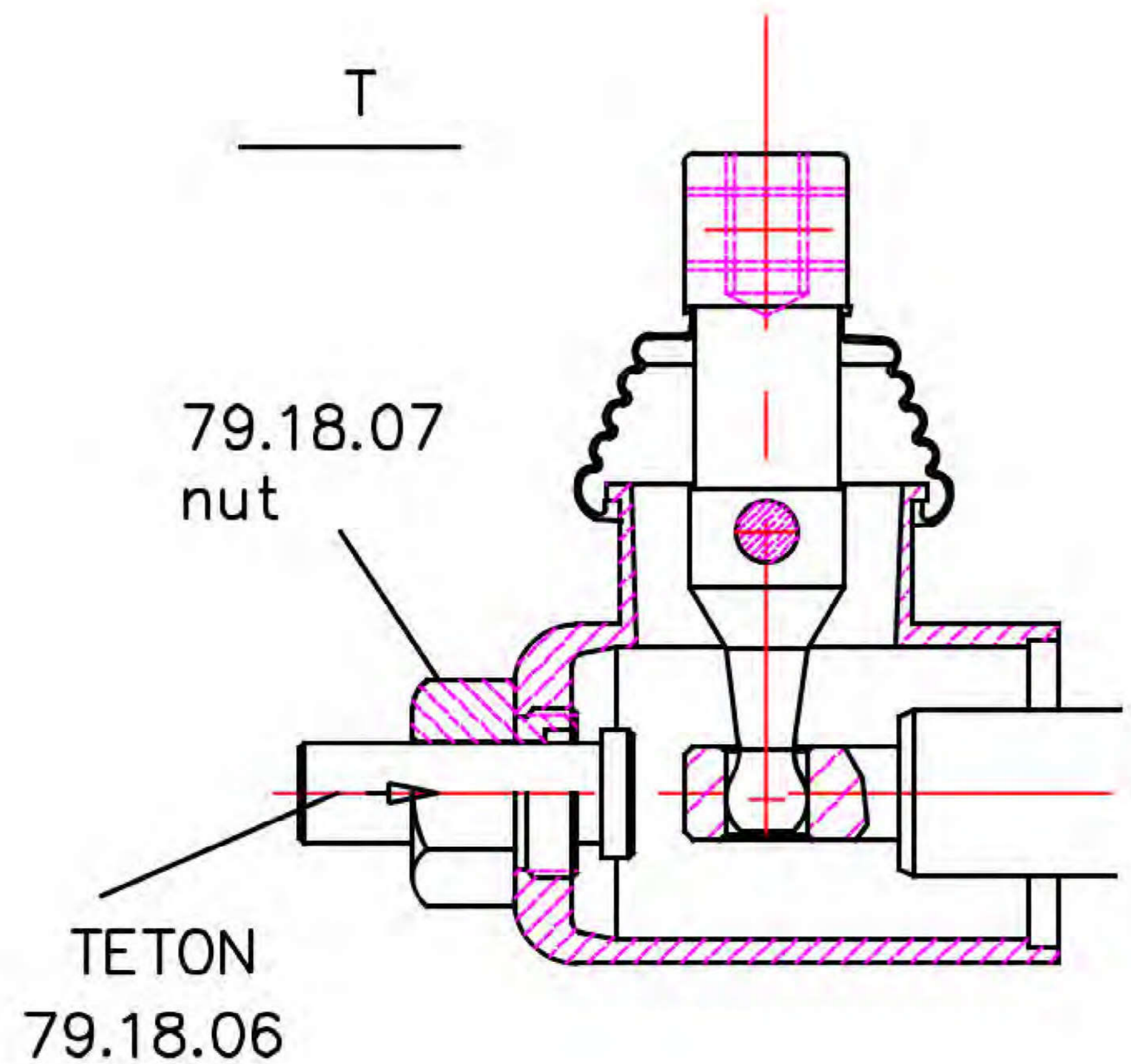
P40 directional control valve
