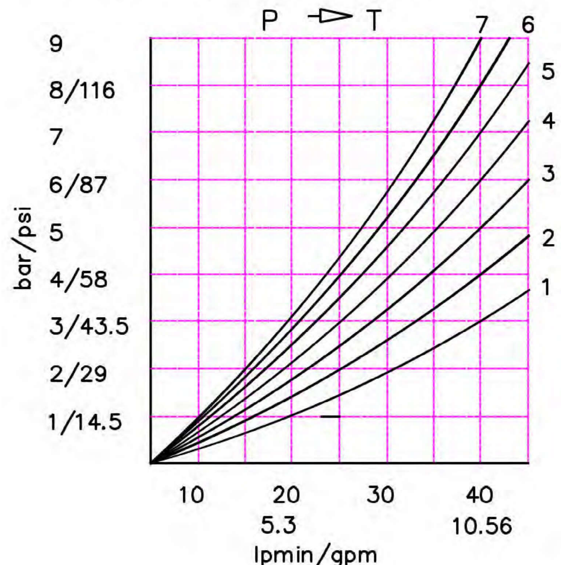
P40 directional control valve
